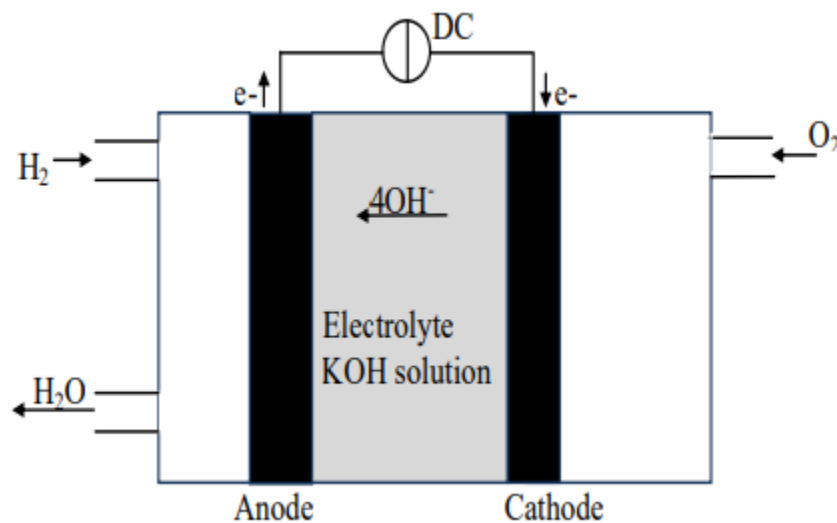
Figure 28. AFC Structure
