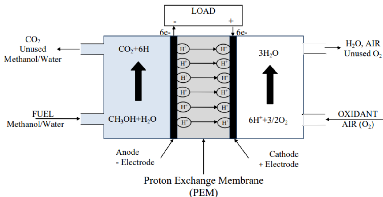
Figure 27. DMFC Structure
